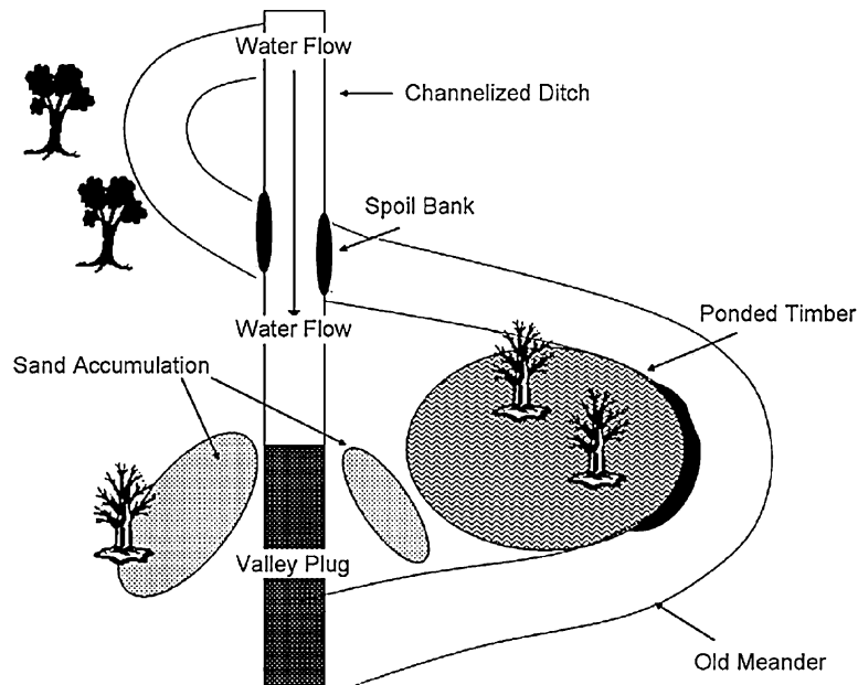
Fig. 1. Generalized map of alluvial system affected by excessive sedimentation and valley plug formation. Atypical geomorphic features are indicated.
